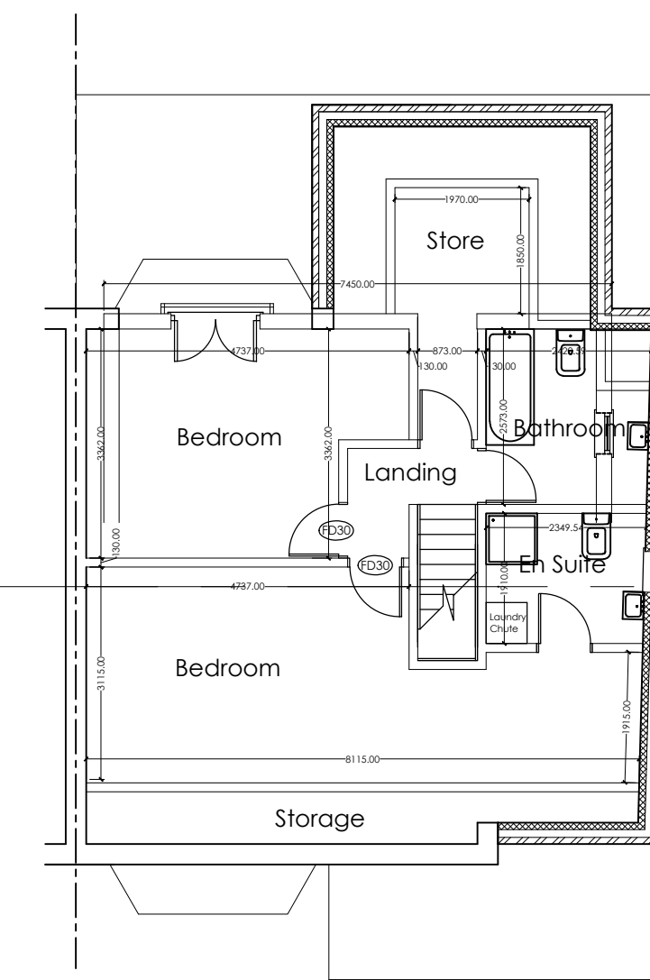
Proposed Second Floor Plan (1 or 2 bedrooms)
