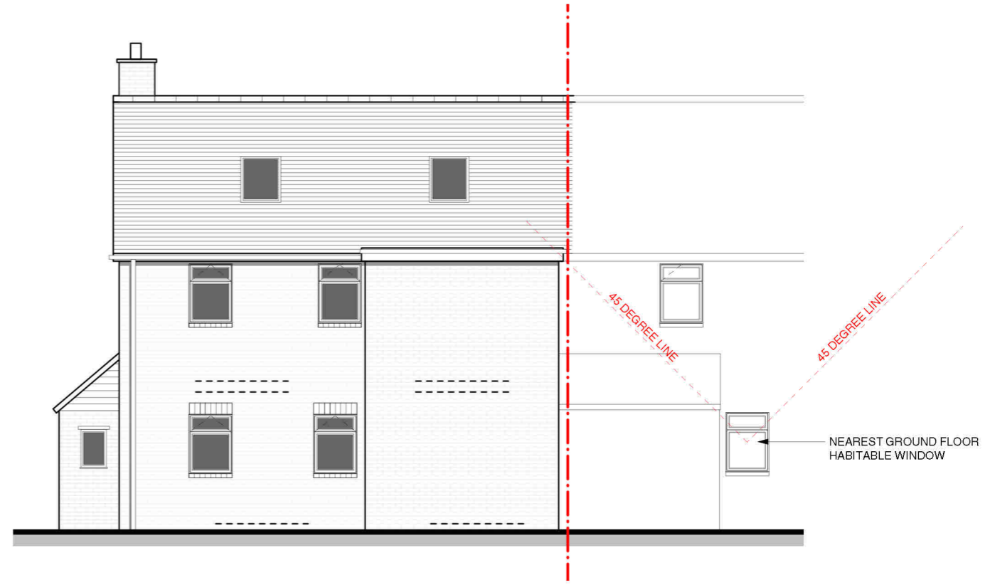
2 PROPOSED REAR ELEVATION 04 SCALE 1:100 @A3
