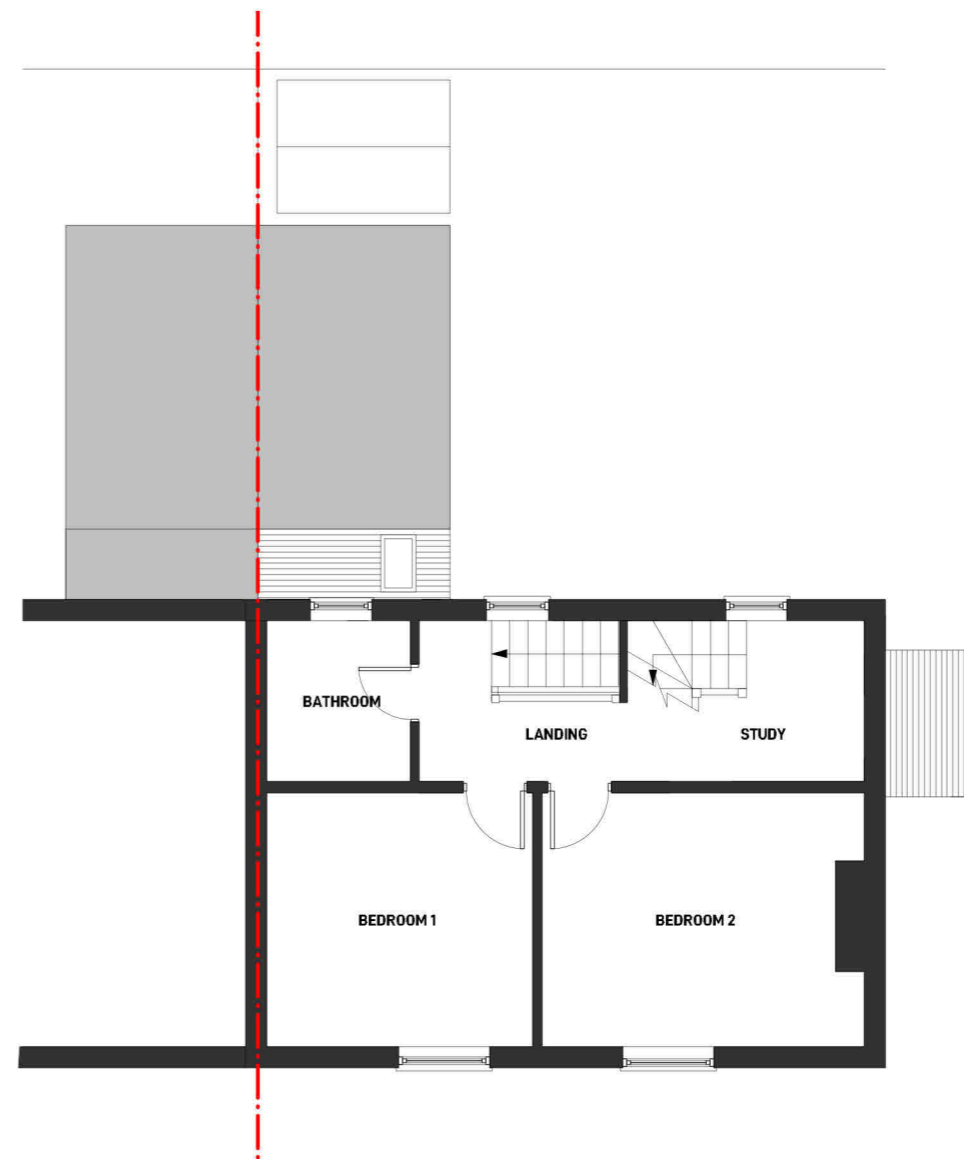
2 01 EXISTING FIRST FLOOR SCALE 1:100 @A3
