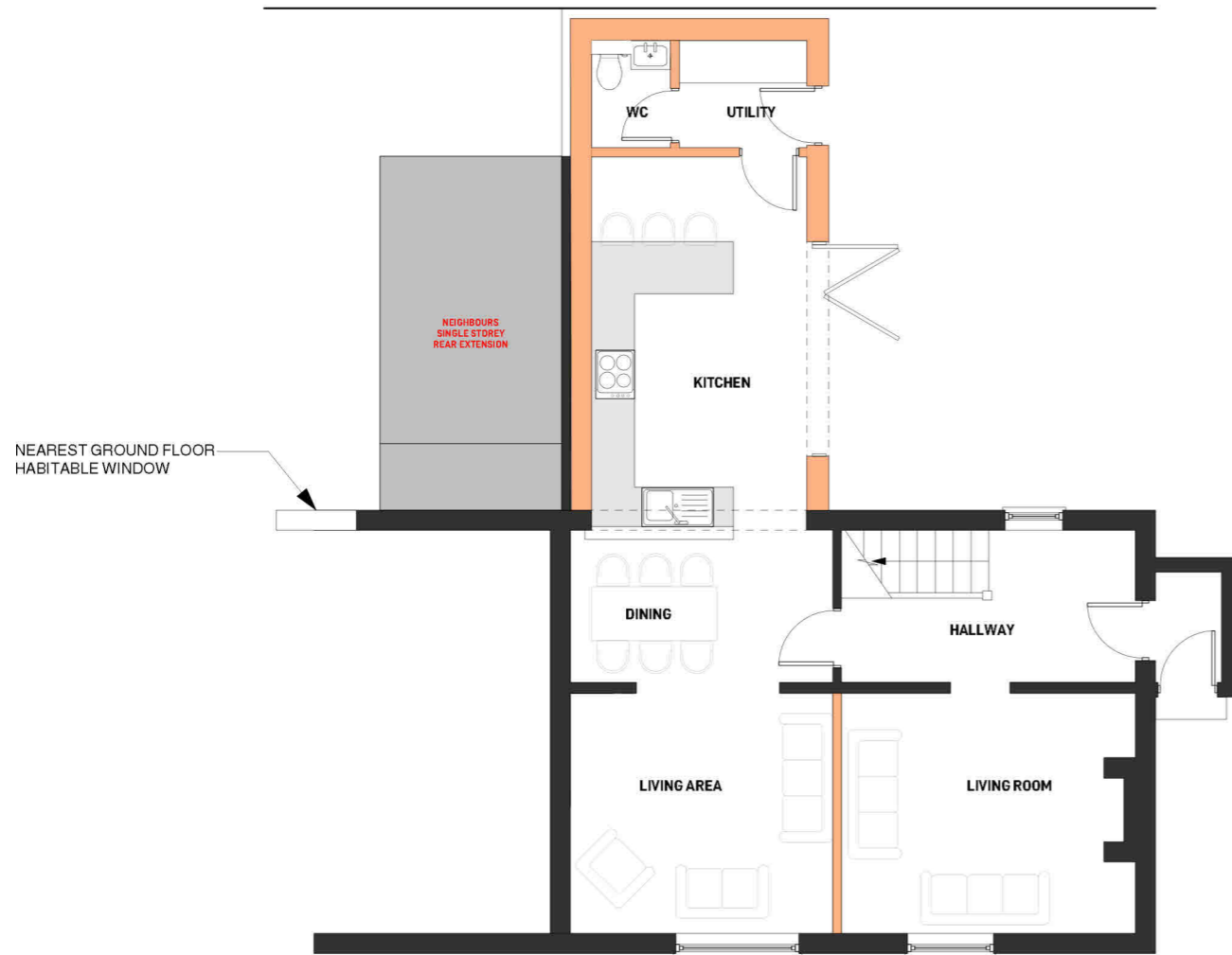
1 PROPOSED GROUND FLOOR 03 SCALE 1:100 @A3
