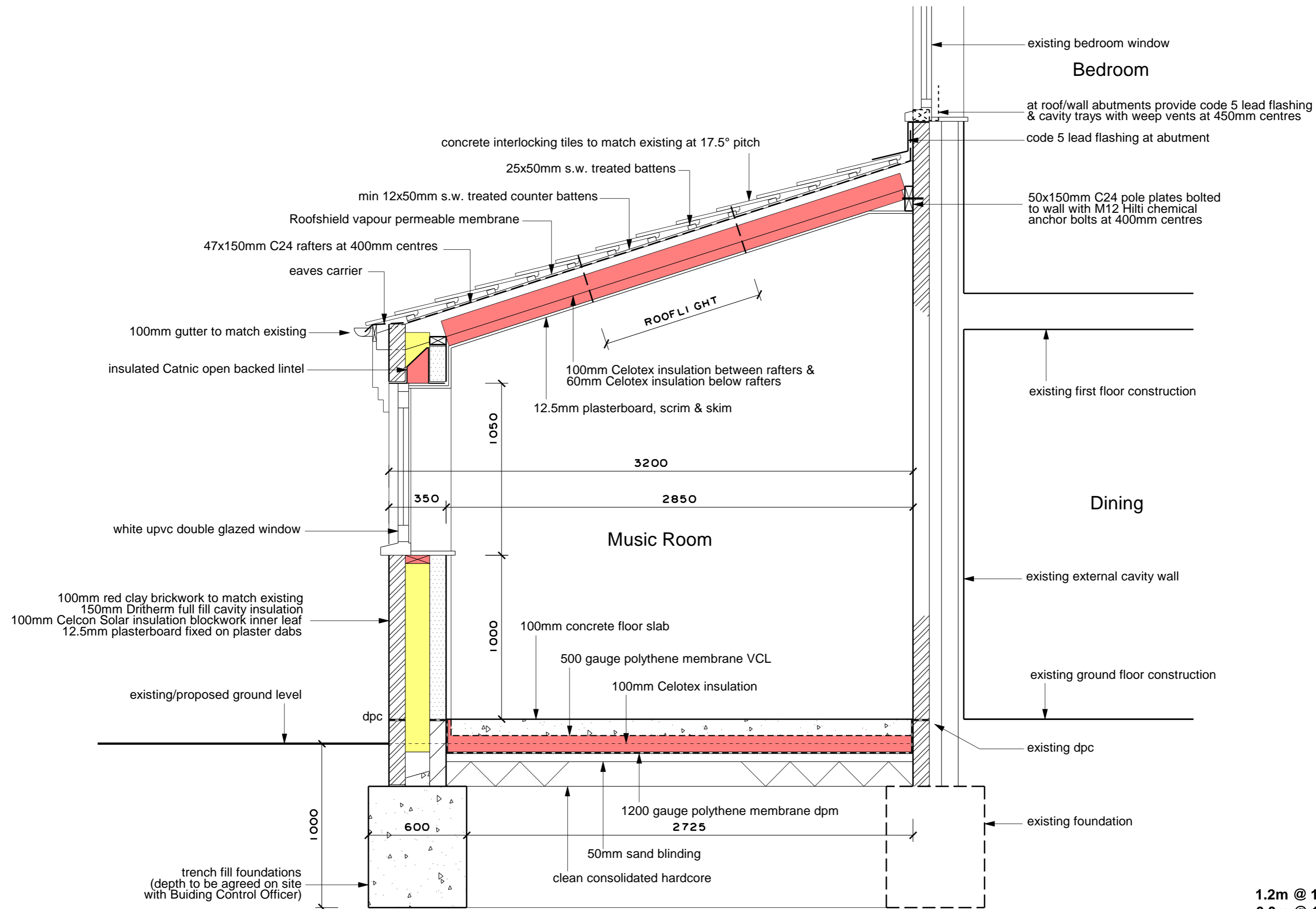
TYPICAL SECTION 1:20
