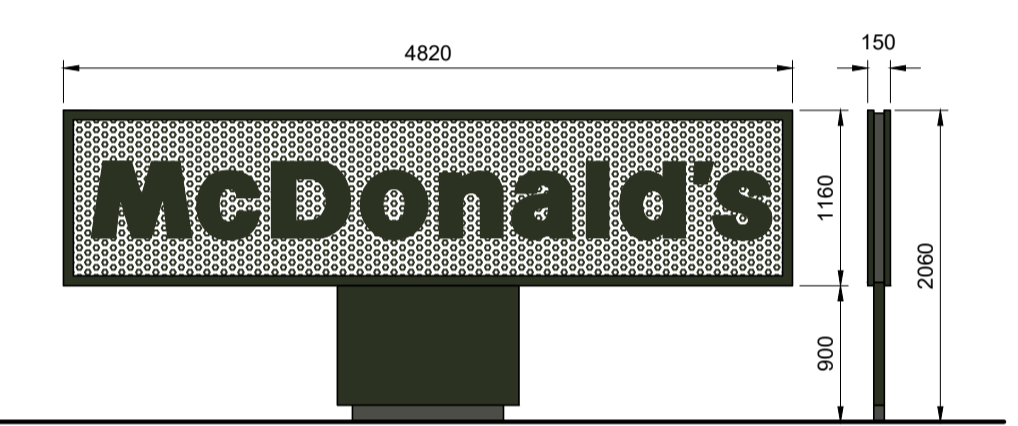
PROPOSED DOUBLE SIDED BANNER UNIT SCALE 1:50
