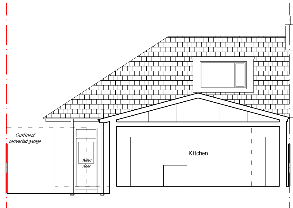
4 Section B-B As Proposed
