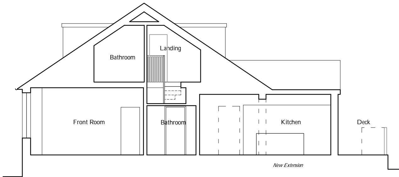
3 Section A-A As Proposed
