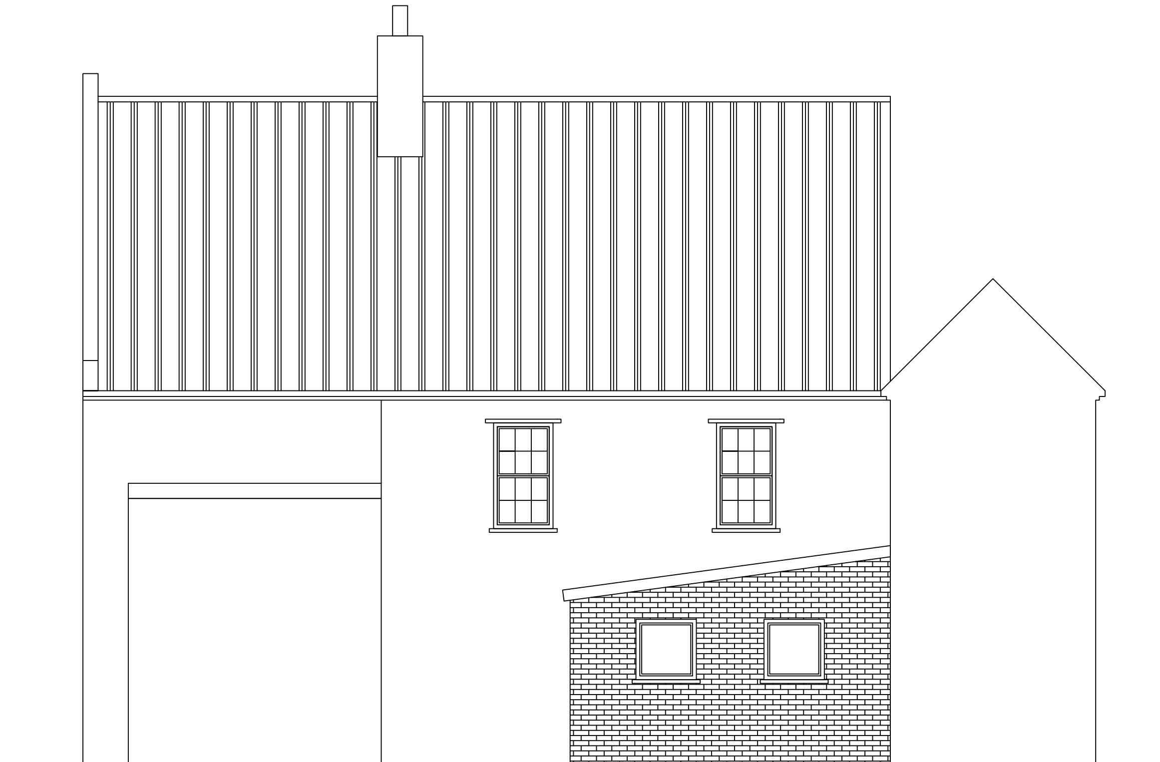
REAR ELEVATION PROPOSED 1:50
