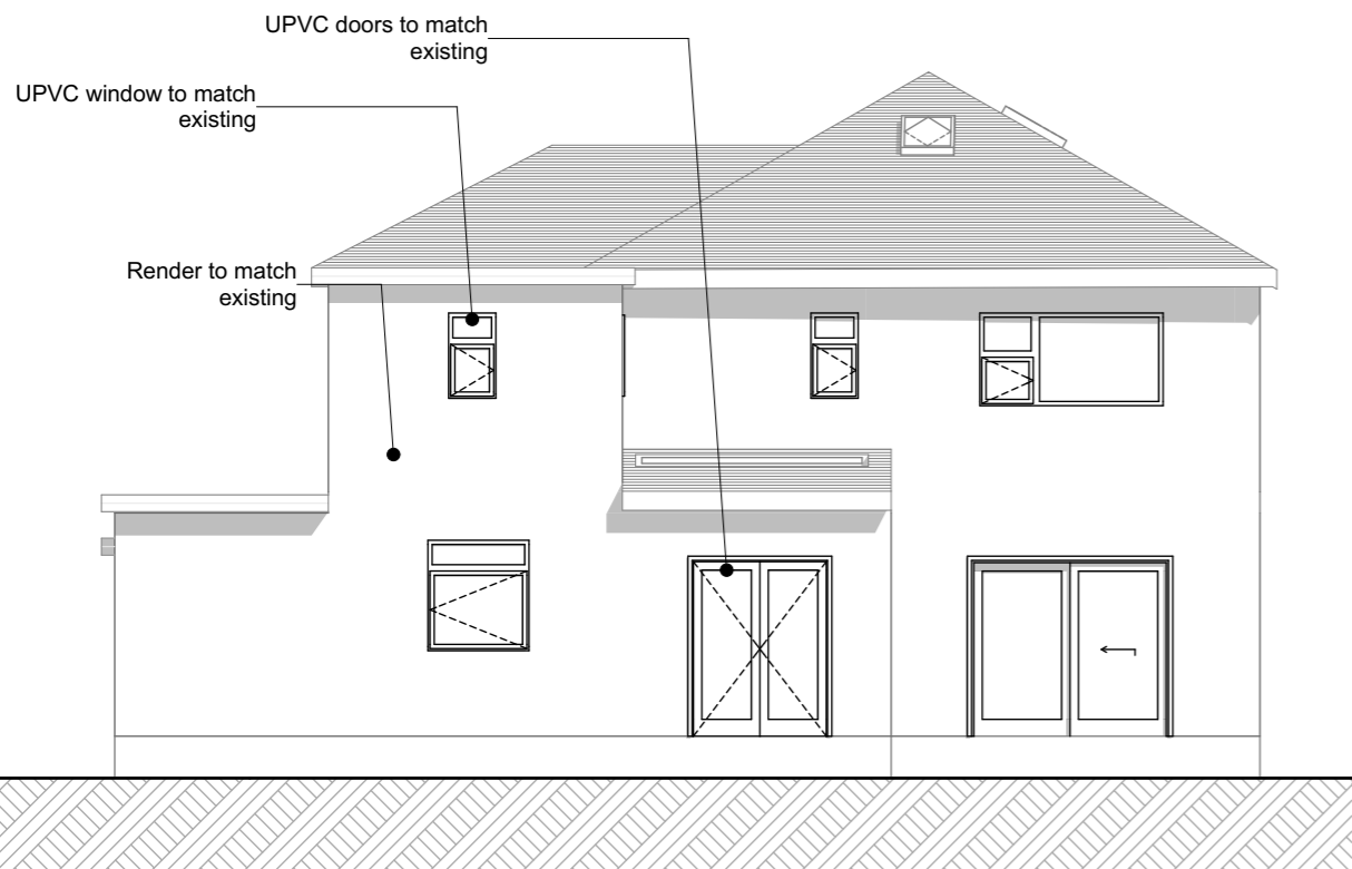
Rear Elevation
