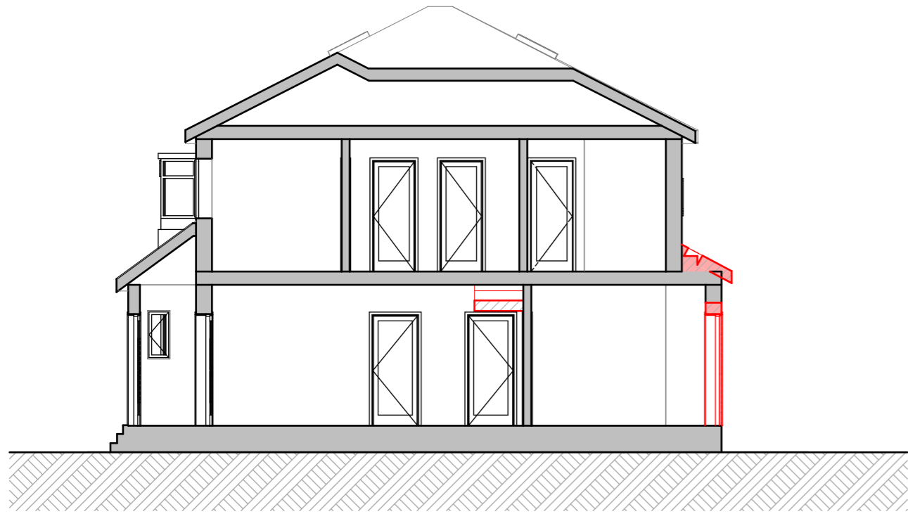
S-01 Section
