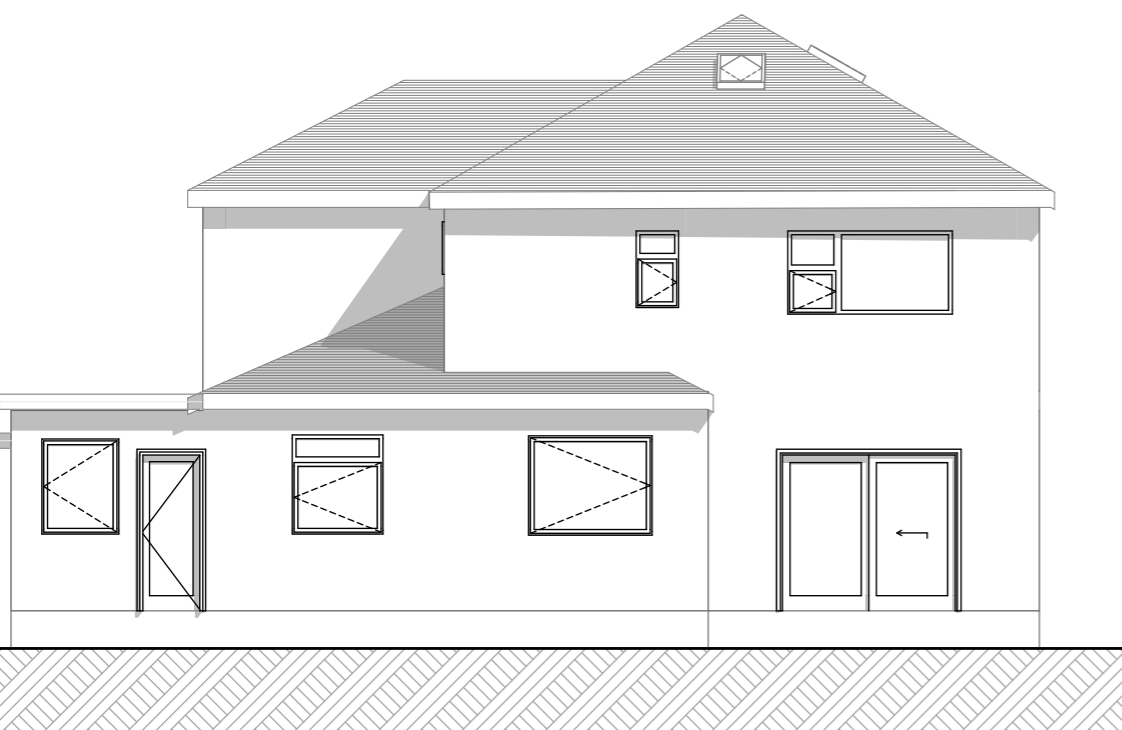
Rear Elevation
