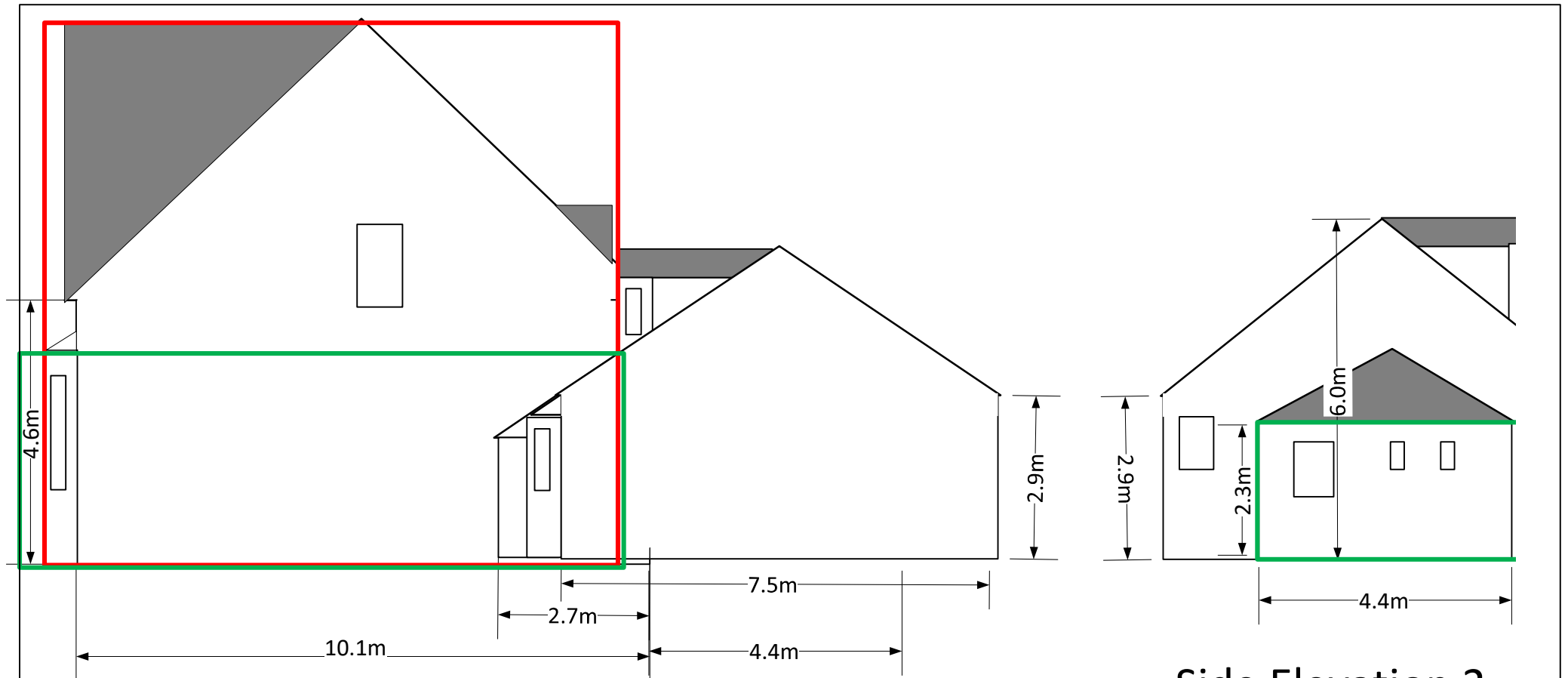
Side Elevation 1
