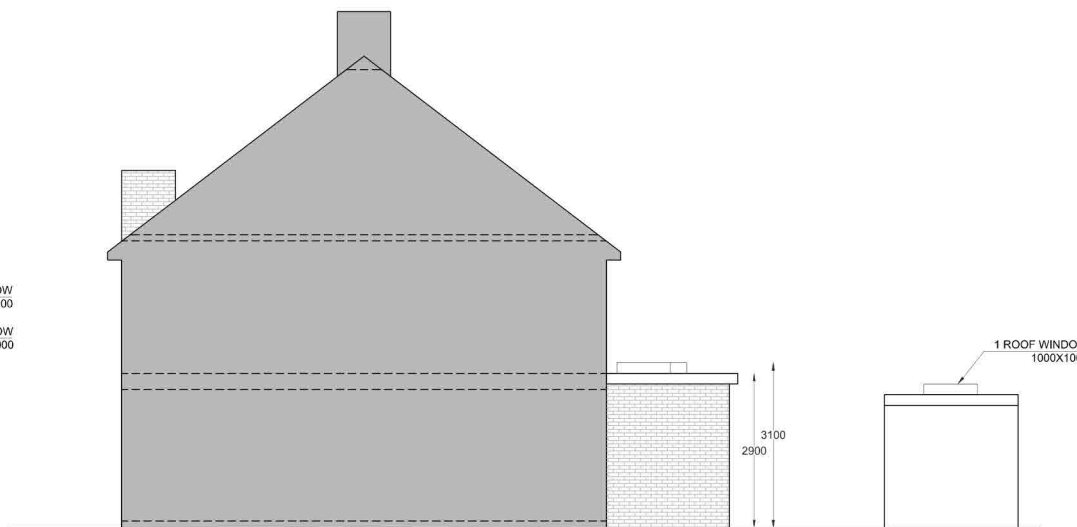
PROPOSED RIGHT ELEVATION
