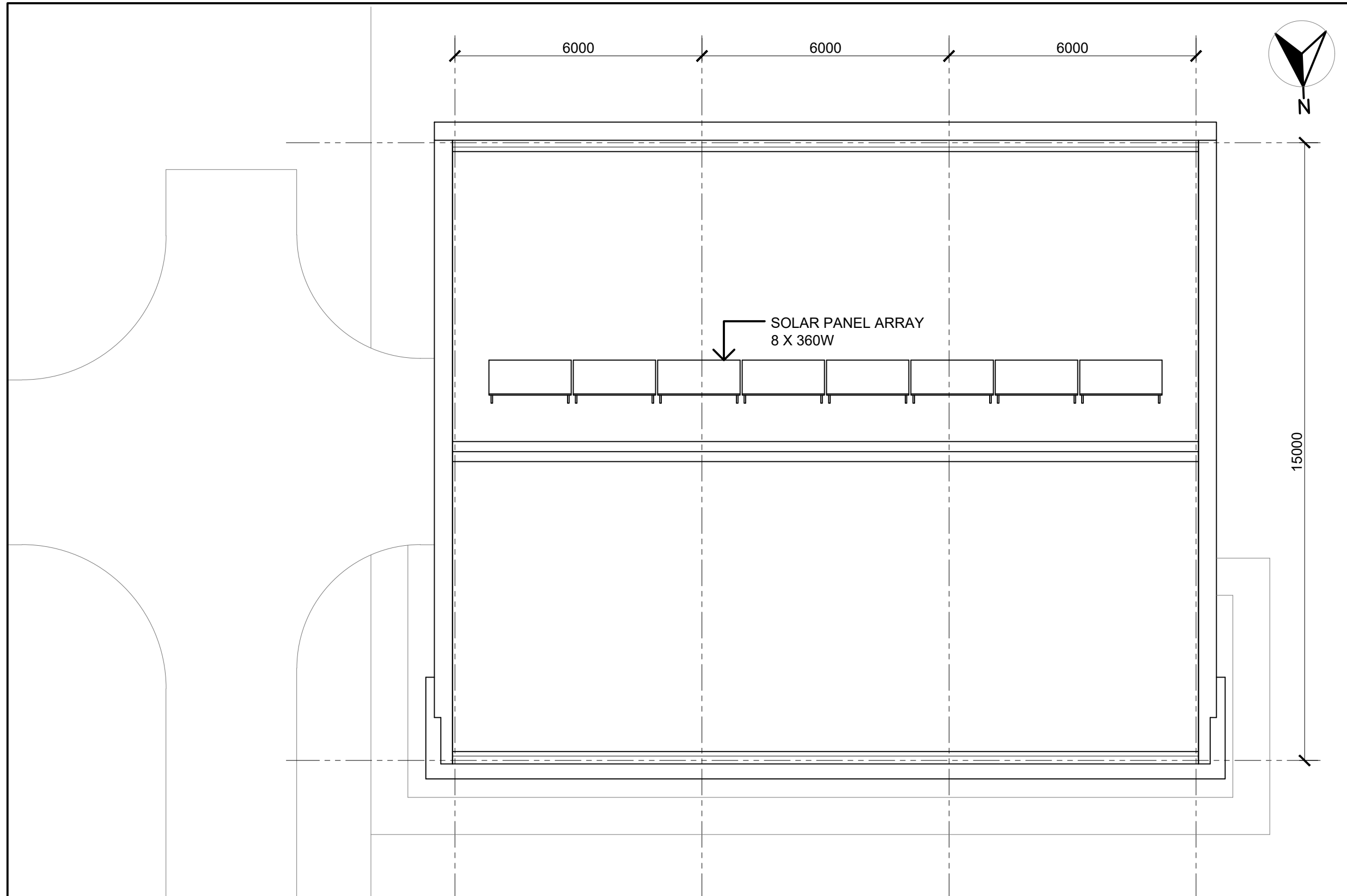
1 FLOOR PLAN
