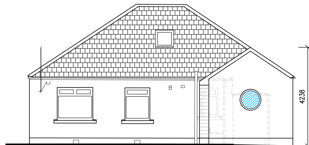
Proposed South East Elevation
