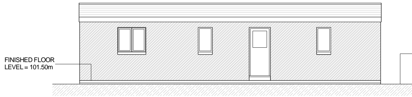
REAR (NORTH) ELEVATION
