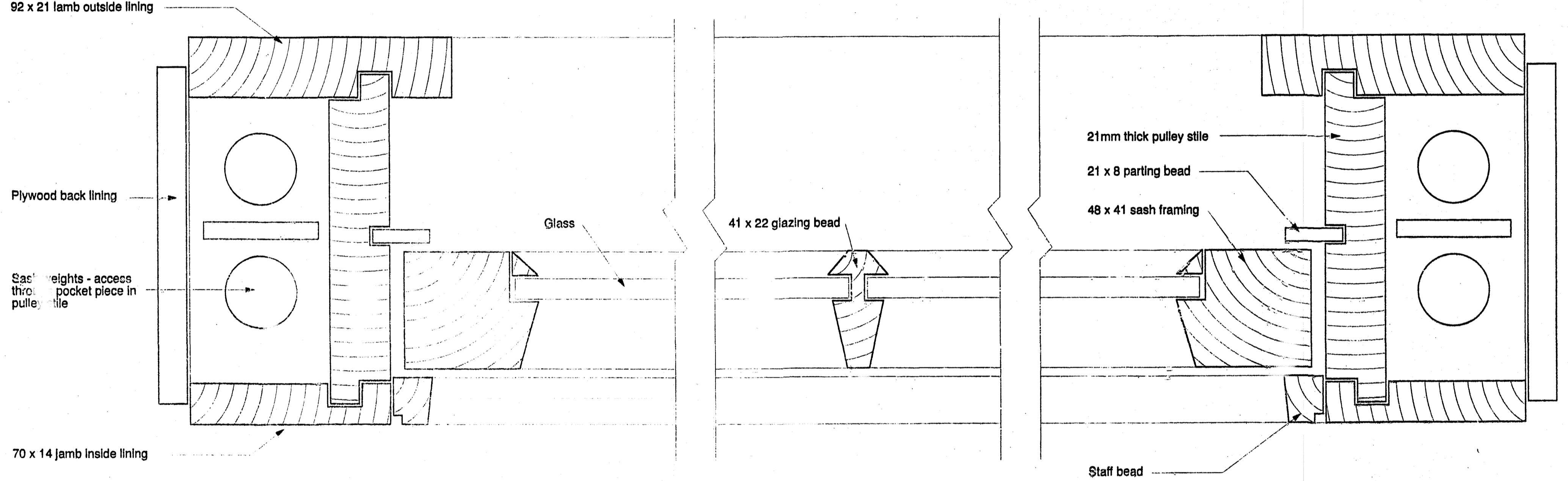
Typical Horizontal Section 1 : 1. Patent Stormproofing seals to meeting rails and sash framing by window manufacturer TIMBER GLAZING BEADS HERITAGE SLIMLINE DOUBLE GLAZING
