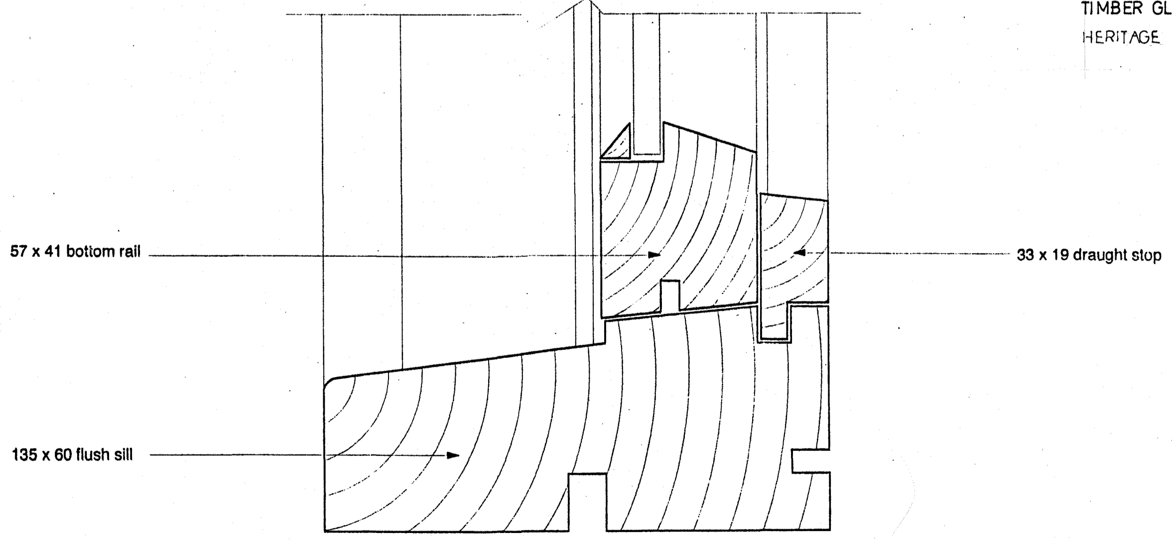
Typical Vertical Section. 1 : 1. Patent Stormproofing seals to meeting rails and sash framing by window manufacturer
