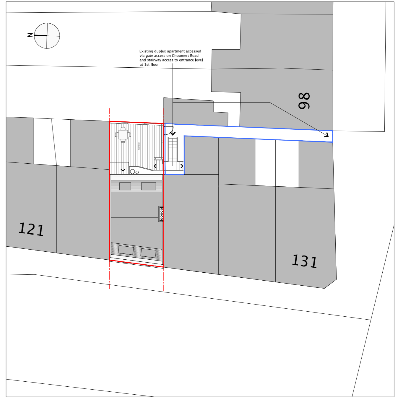
BLOCK PLAN - EXISTING 1:200
