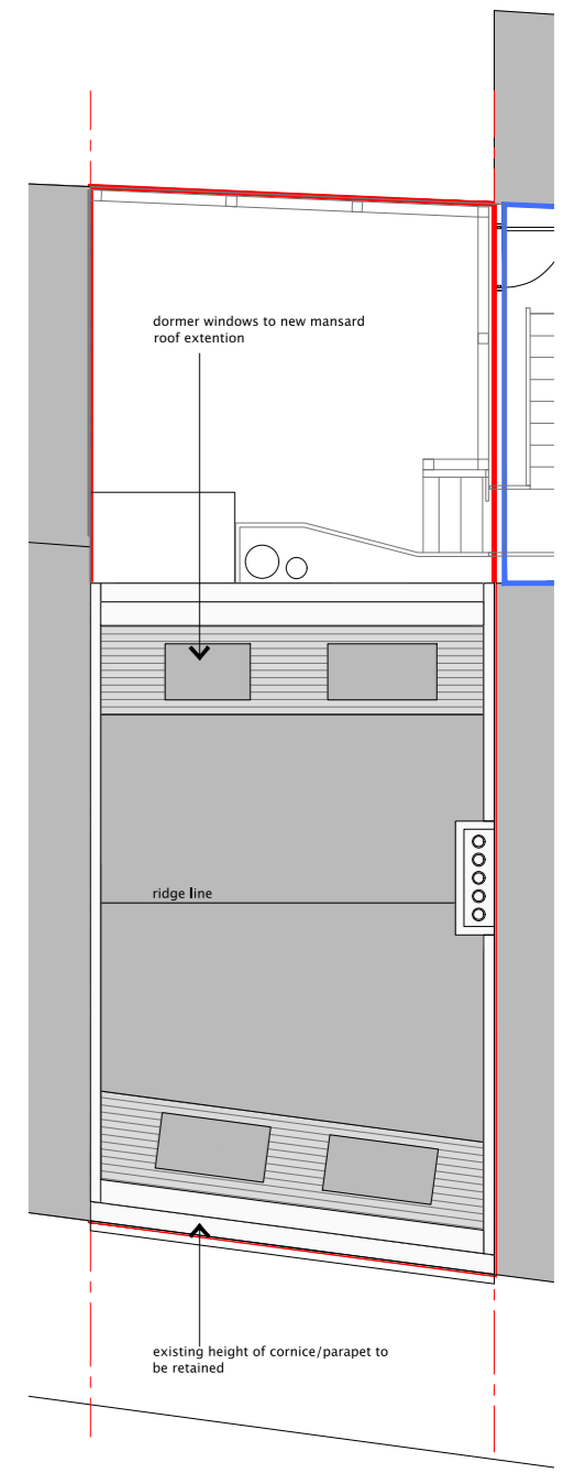
ROOF PLAN – PROPOSED
