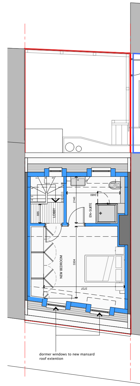
THIRD (ROOF EXTENSION) FLR PLAN PROPOSED
