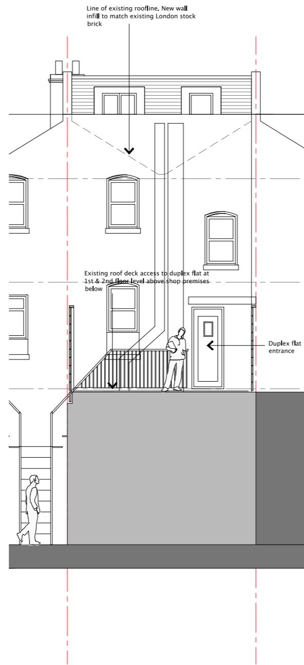
REAR ELEVATION – PROPOSED
