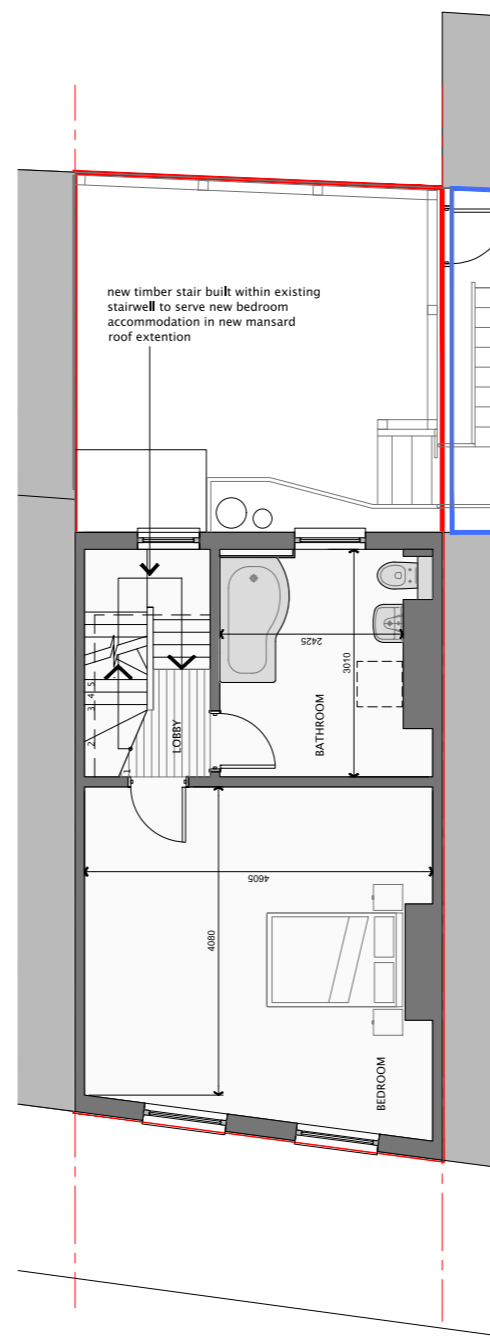
SECOND FLR PLAN – PROPOSED
