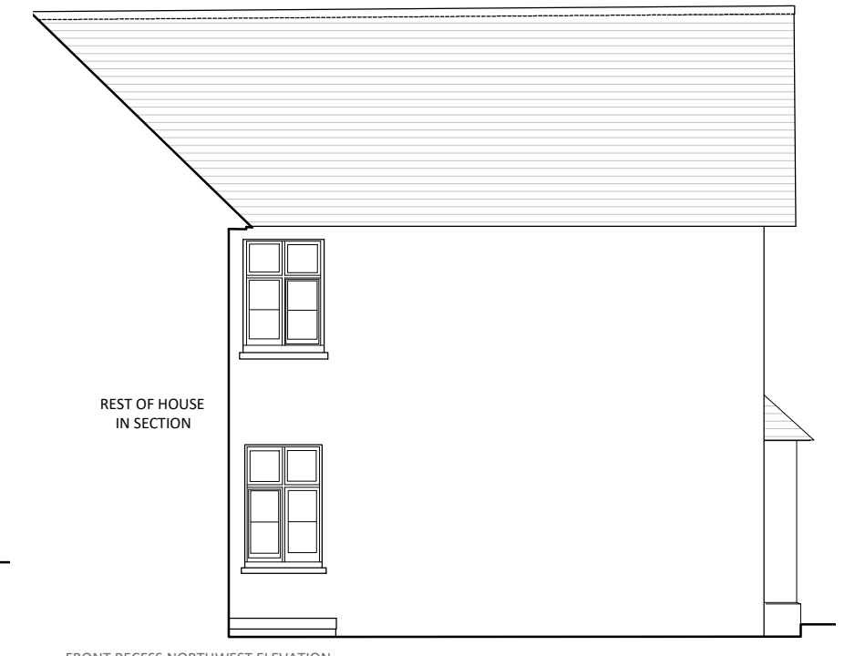
FRONT RECESS NORTHWEST ELEVATION As Existing
