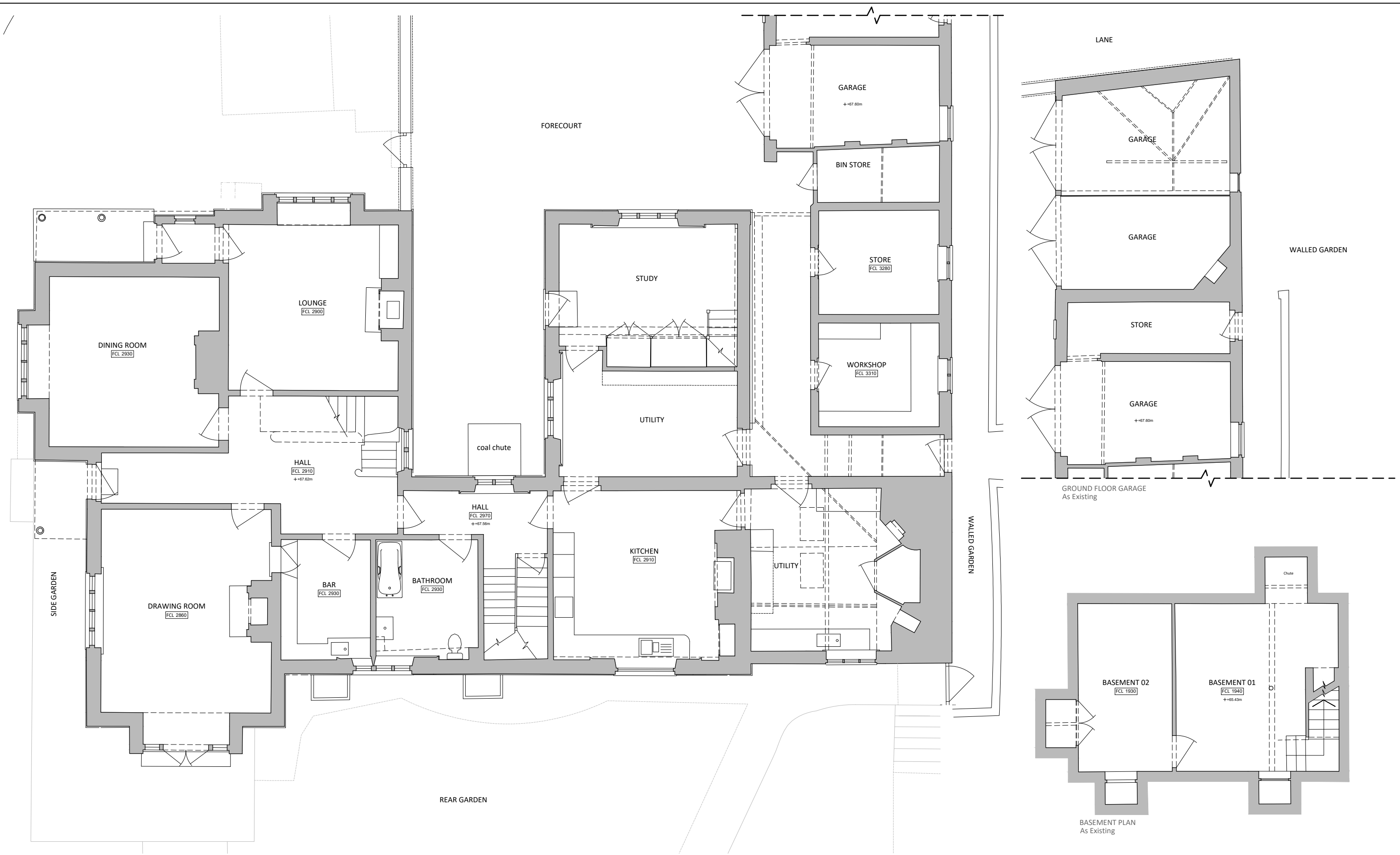
GROUND FLOOR PLAN As Existing
