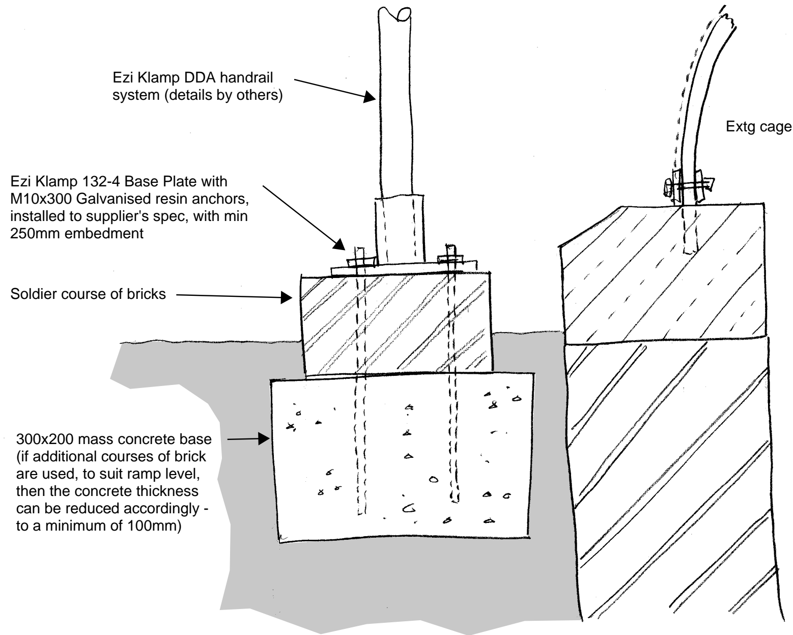
TYPICAL SUPPORT DETAIL
