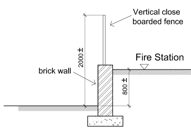
Boundary Detail A-A
