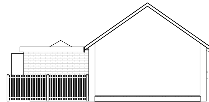
Proposed Elevation-Left side
