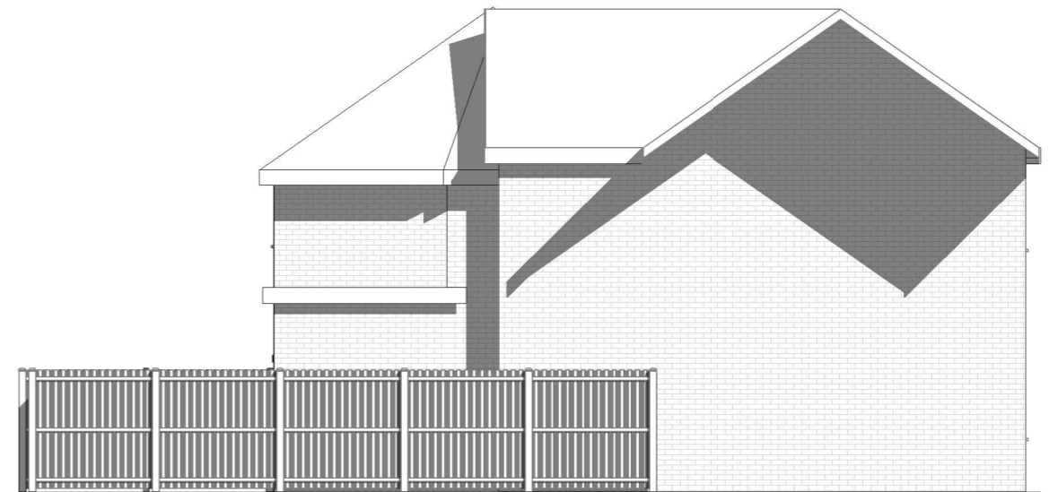
Proposed Elevation-Left side
