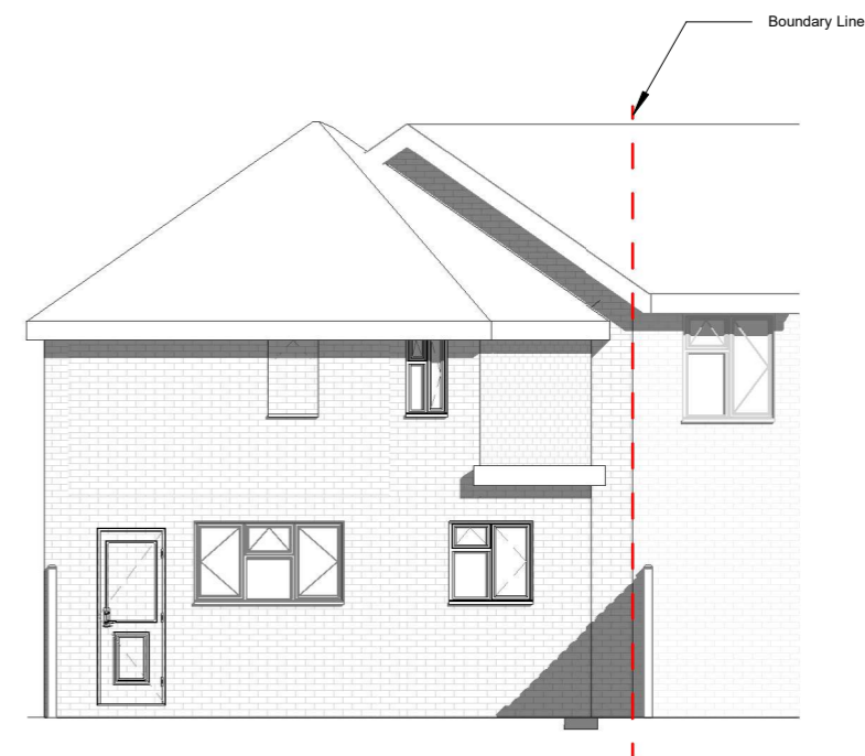
Proposed Elevation-Rear
