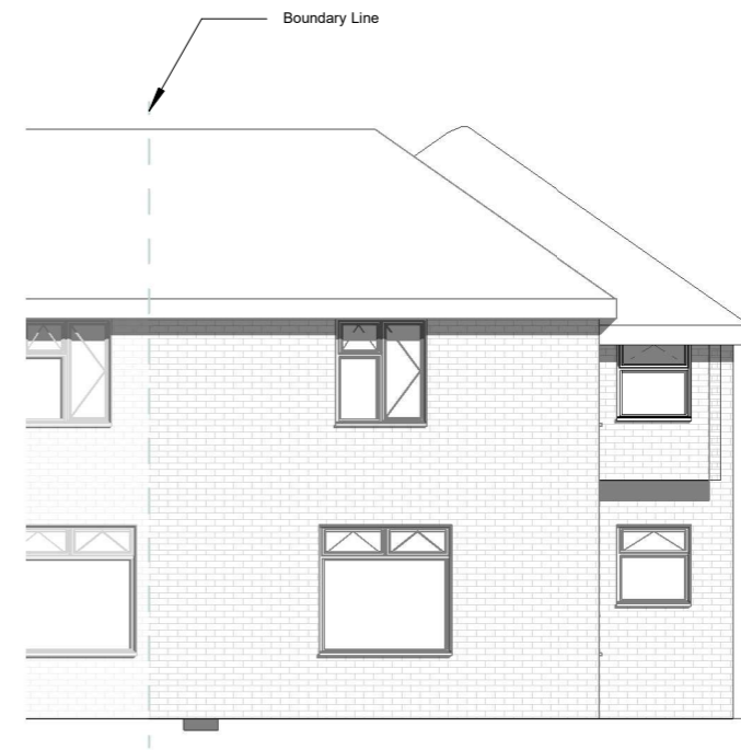
Proposed Elevation-Front
