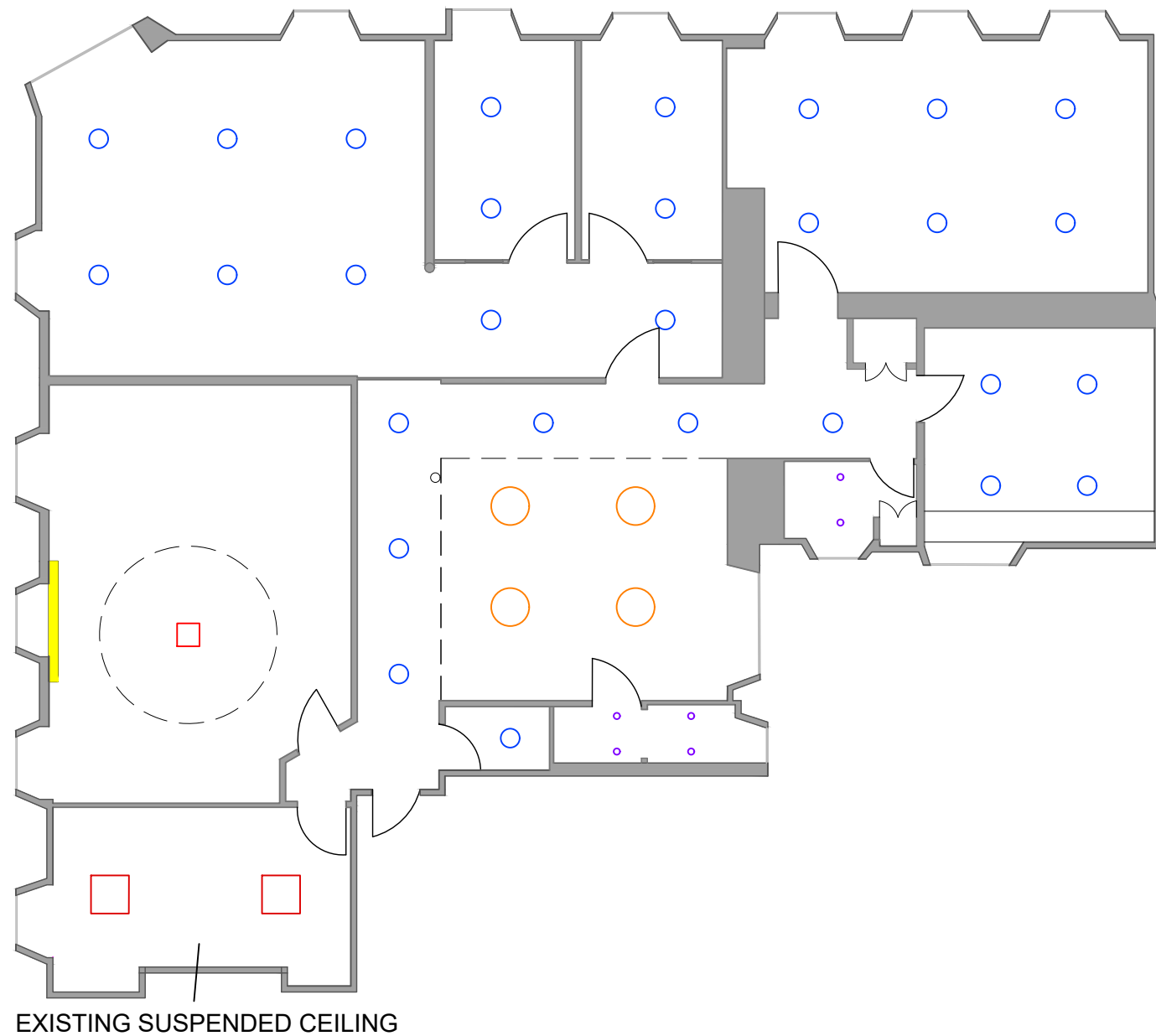
PROPOSED LIGHTING PLAN 1.100
