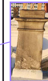
Photograph of chimney pot at party wall with No.19 to be replaced like for like.
