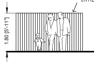
Proposed fence elevation
