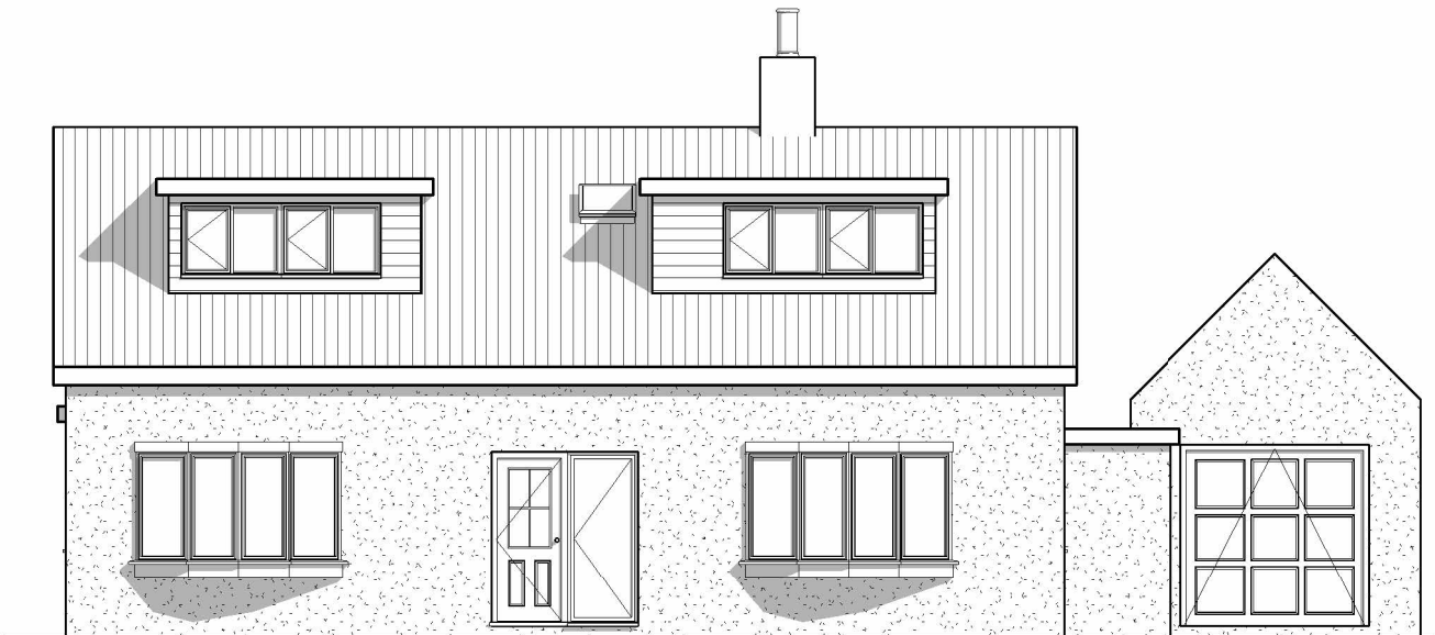
2 Proposed Front 1 : 100
