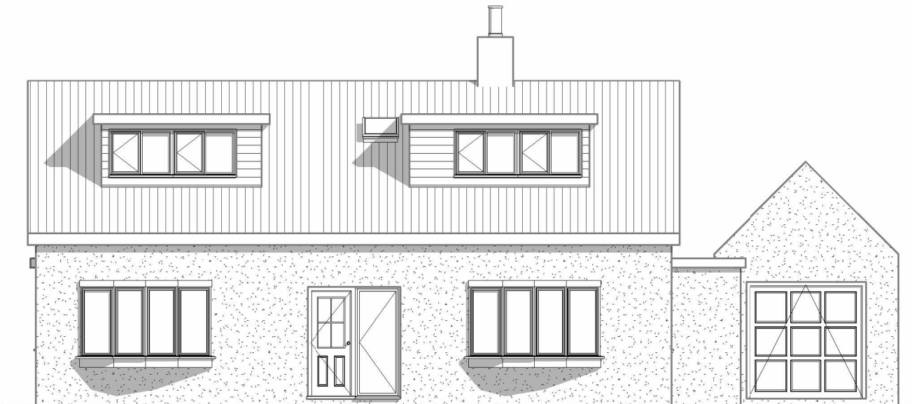
1 Existing Front 1 : 100
