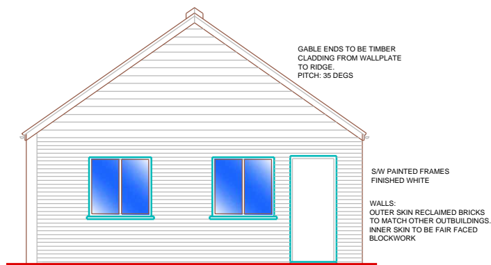
SOUTH EAST (SIDE) ELEVATION
