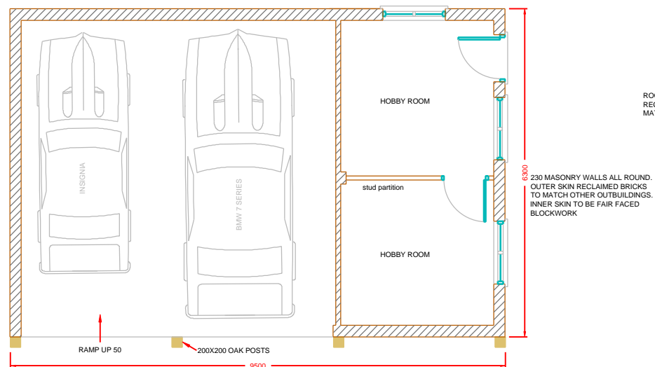
PROPOSED PLAN
