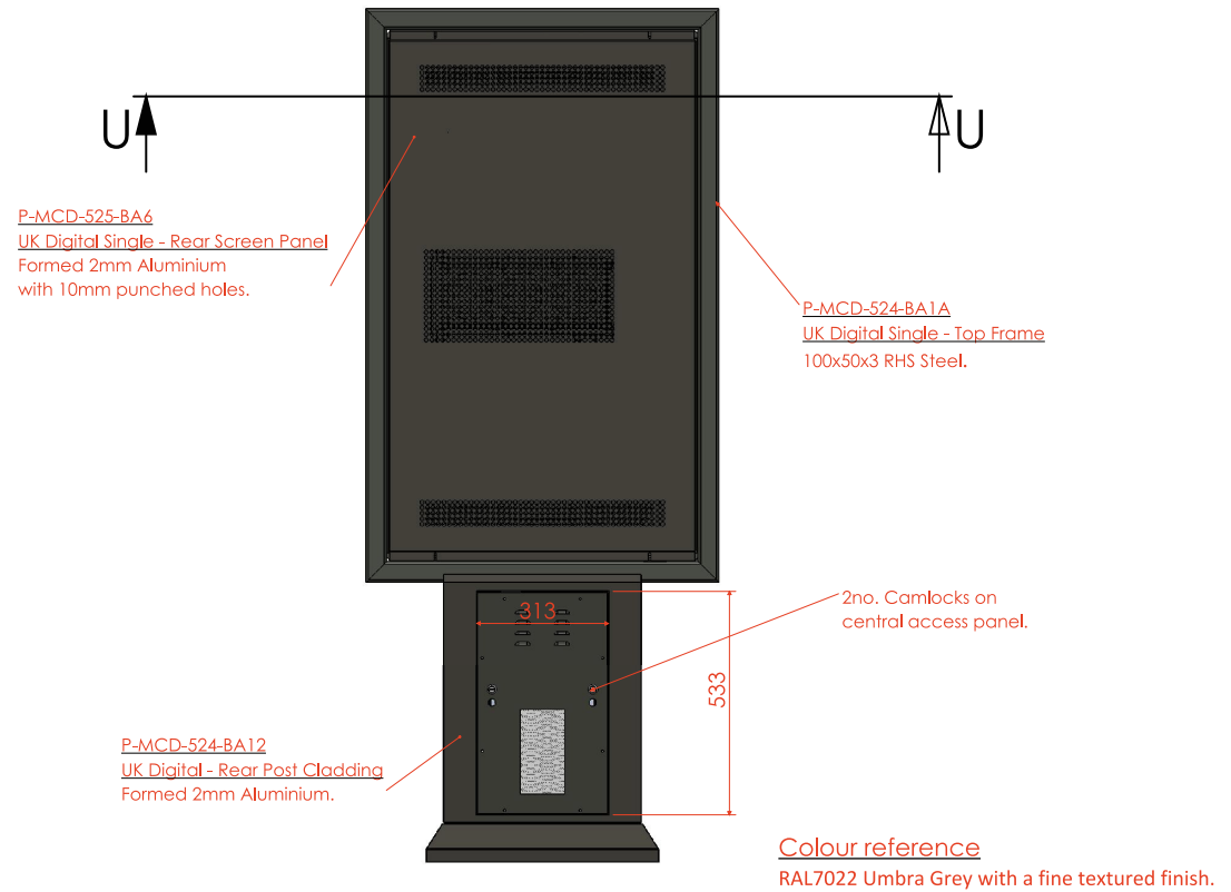
Rear View
