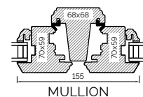
MULLION
