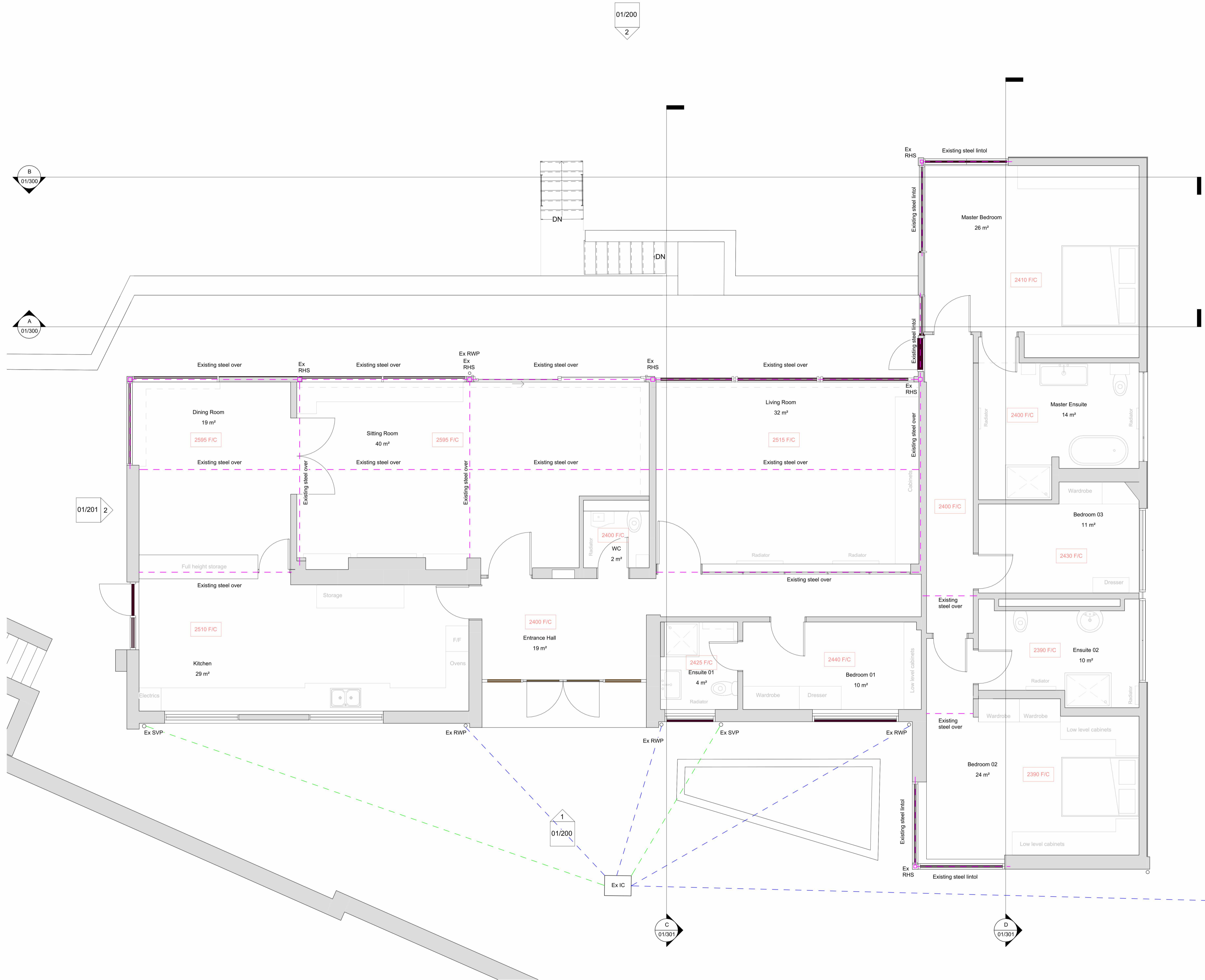
1 Existing Ground Floor Plan 1 : 50
