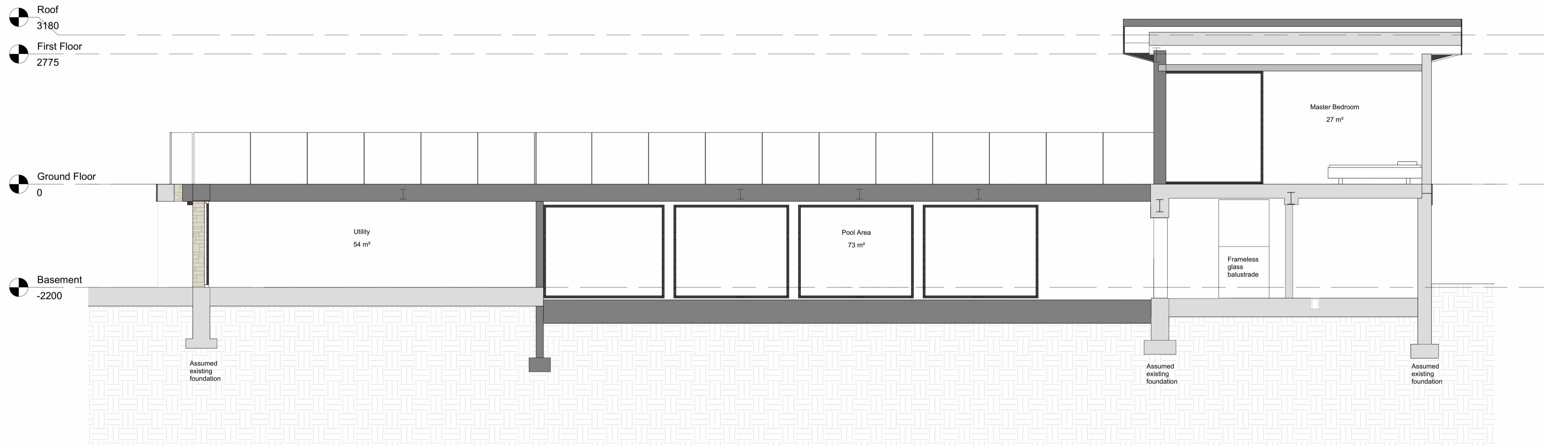
A Proposed Section A 1 : 50
