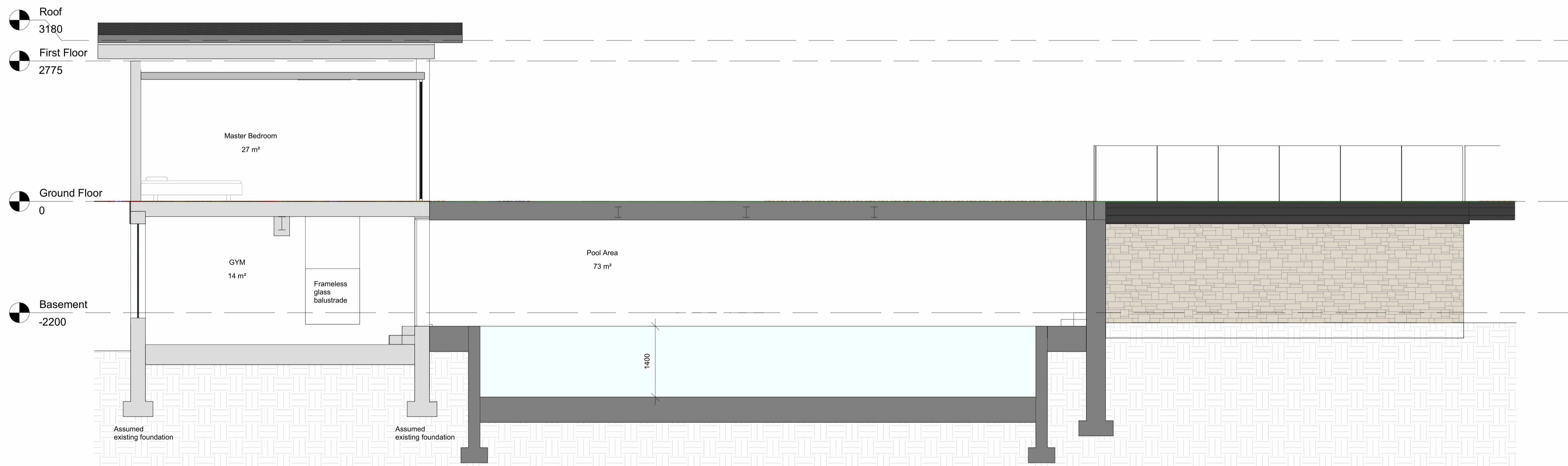
B Proposed Section B 1 : 50
