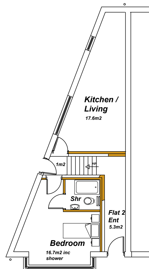
Proposed Ground Floor Plan Scale 1:100 44a
