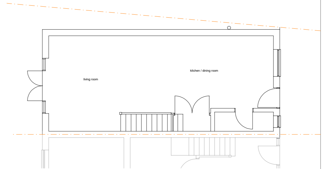
EXISTING GROUND FLOOR PLAN 1:100
