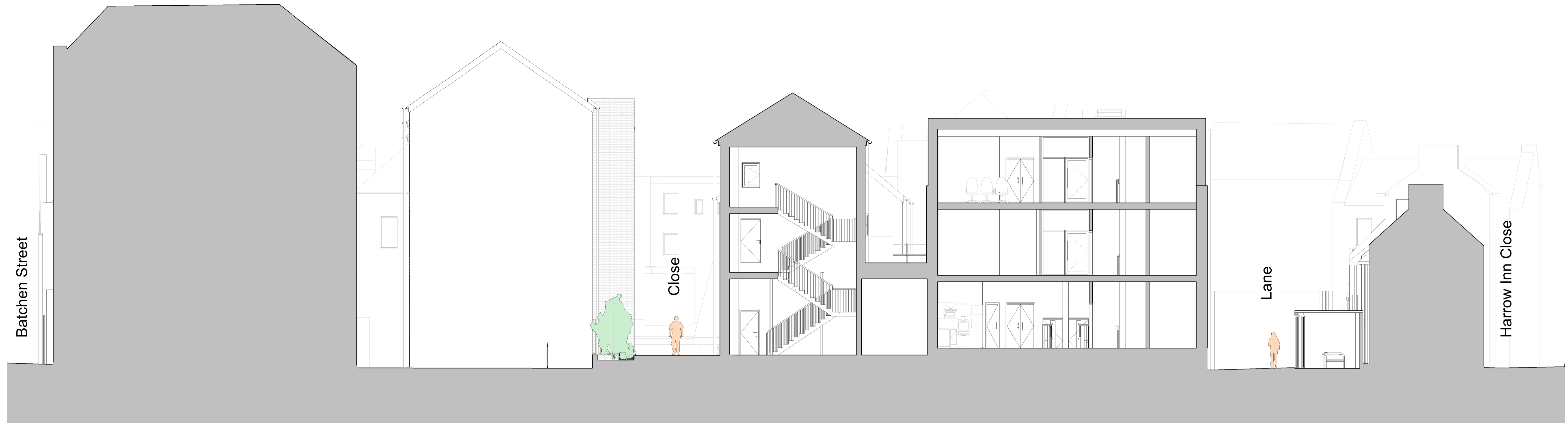
Section 1 - Looking North 1 : 100
