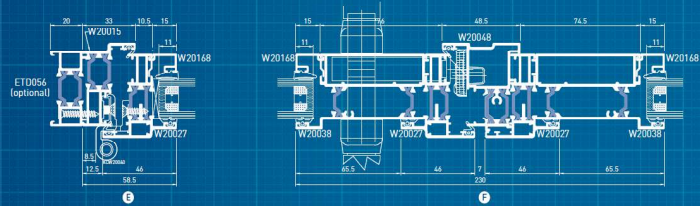
HORIZONTAL SECTION THROUGH LOCK
