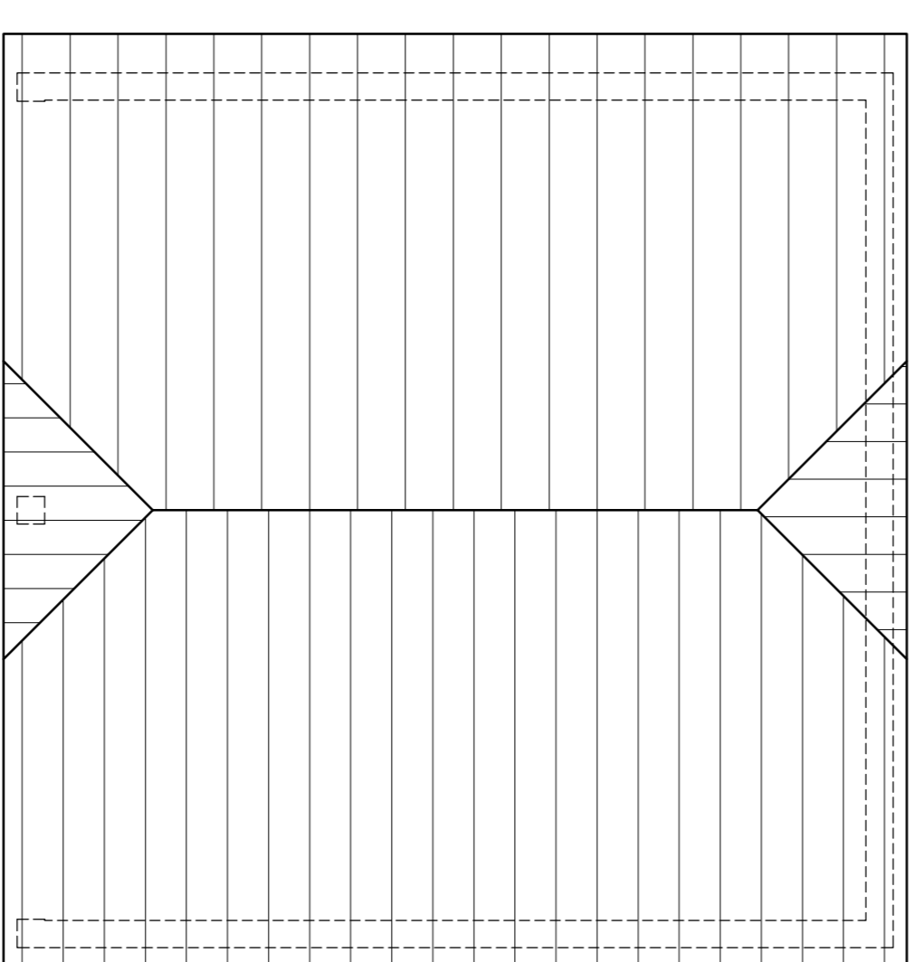
PROPOSED CARPORT ROOF PLAN
