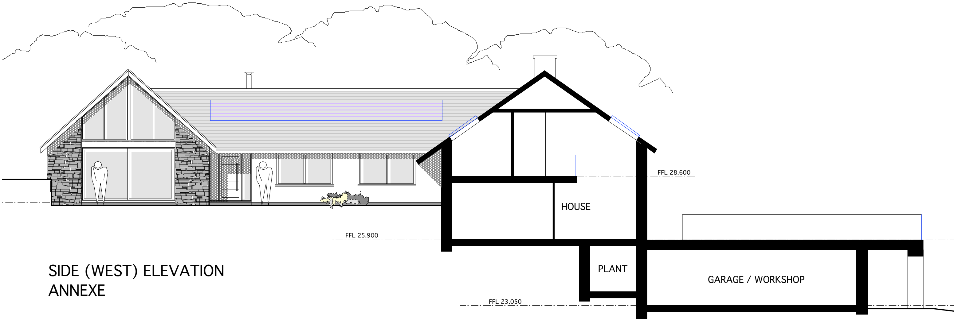
CROSS SECTION HOUSE
