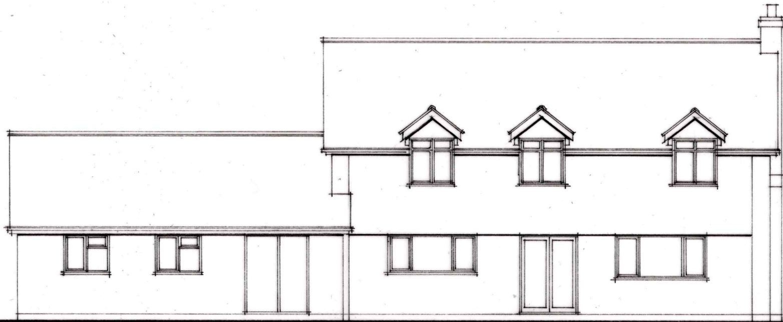
front elevation. 1:100.
