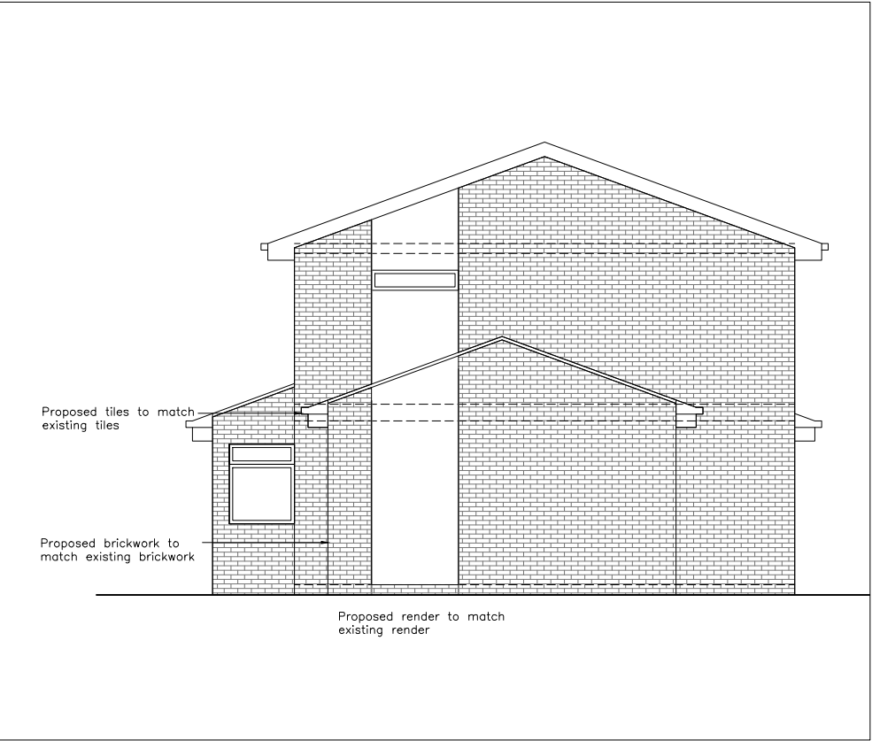
FRONT ELEVATION
