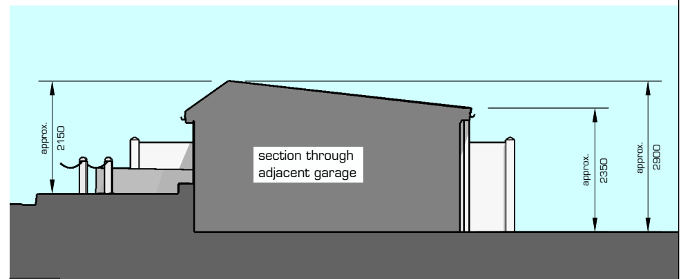
e section looking southeast 005 scale: 1:100
