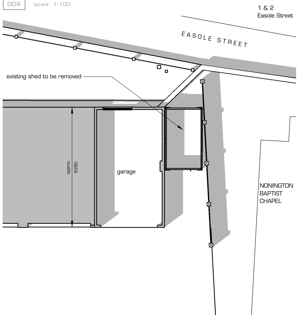
f ground floor plan 006 scale: 1:100
