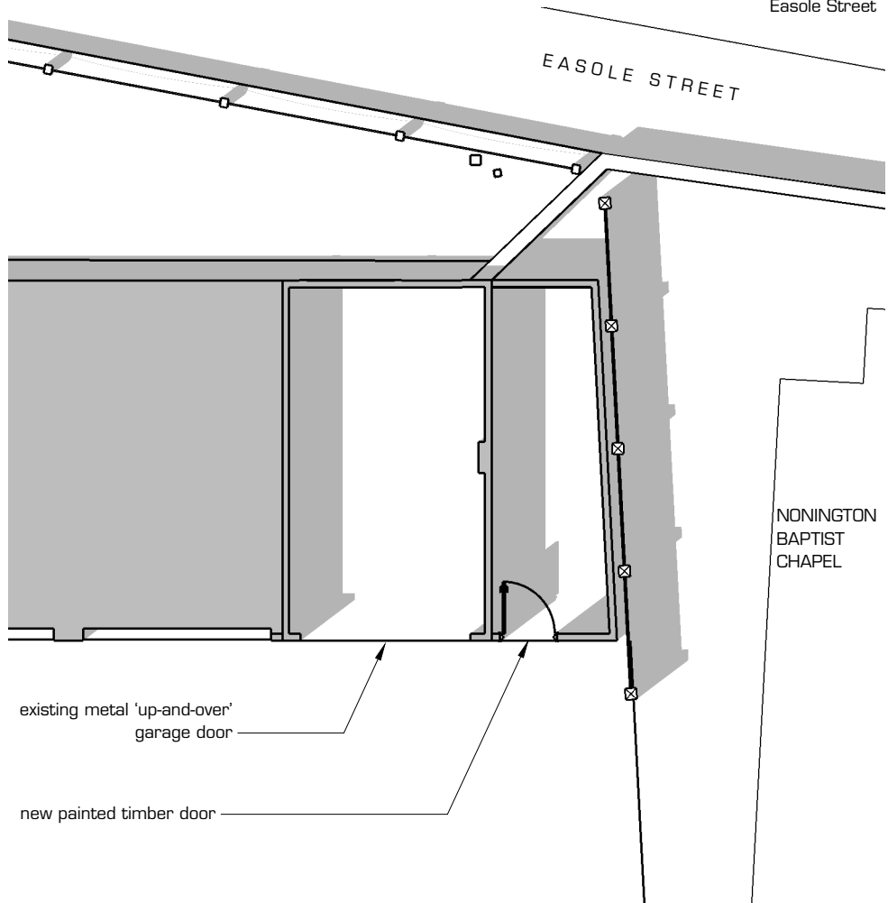
f ground floor plan 006 scale: 1:100
