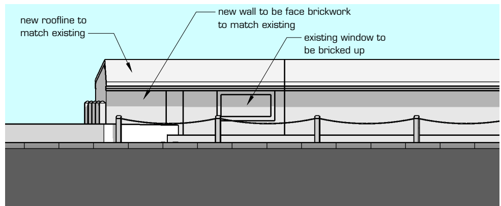
d northeast (street) elevation 004 scale: 1:100
