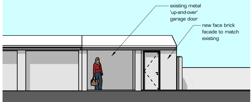
b southwest (front) elevation 002 scale: 1:100
