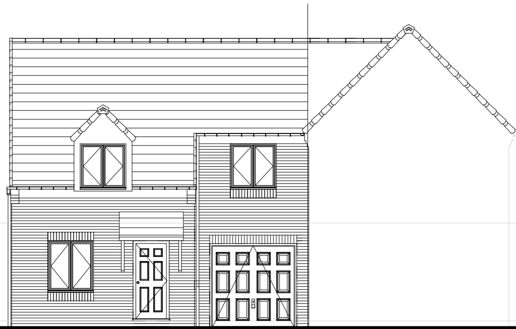
FRONT ELEVATION
