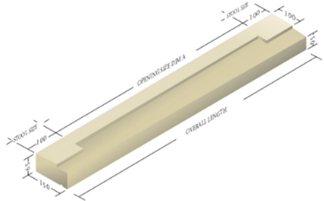
Masonry Detailing – Buff wet-cast stone cills to match existing
