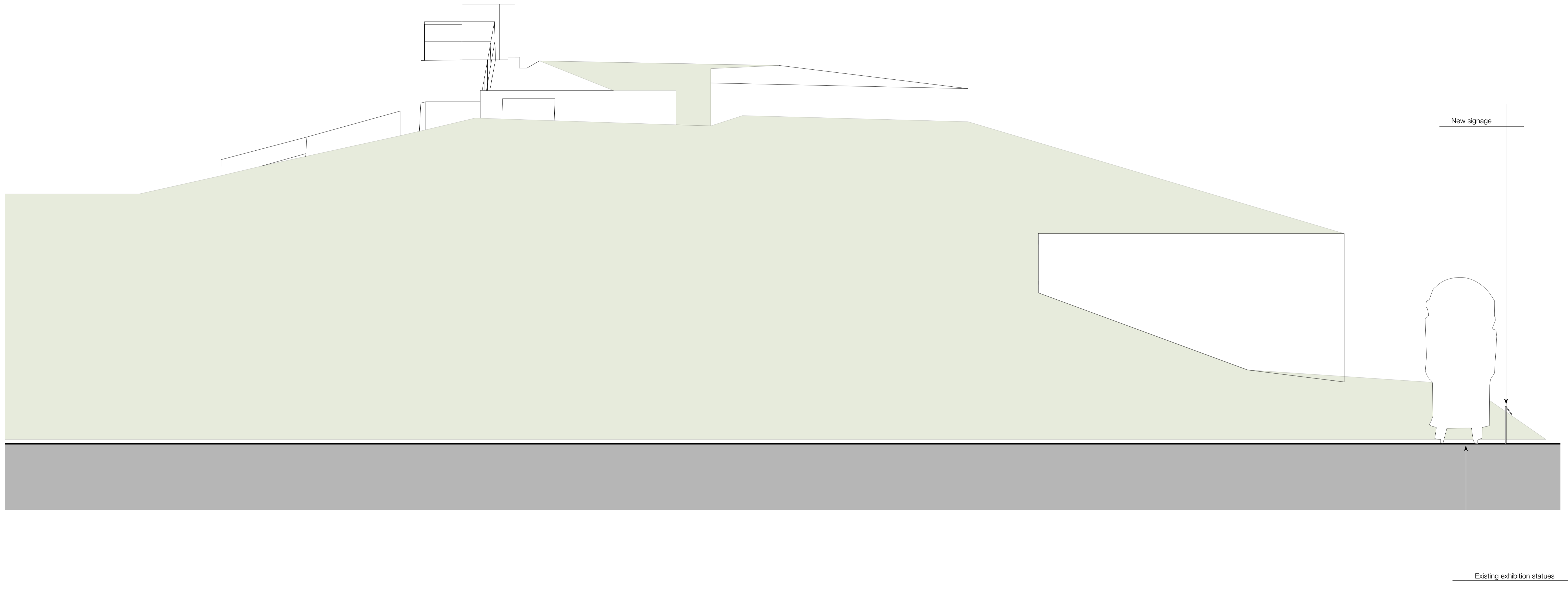
Proposed West Elevation Scale 1:50
