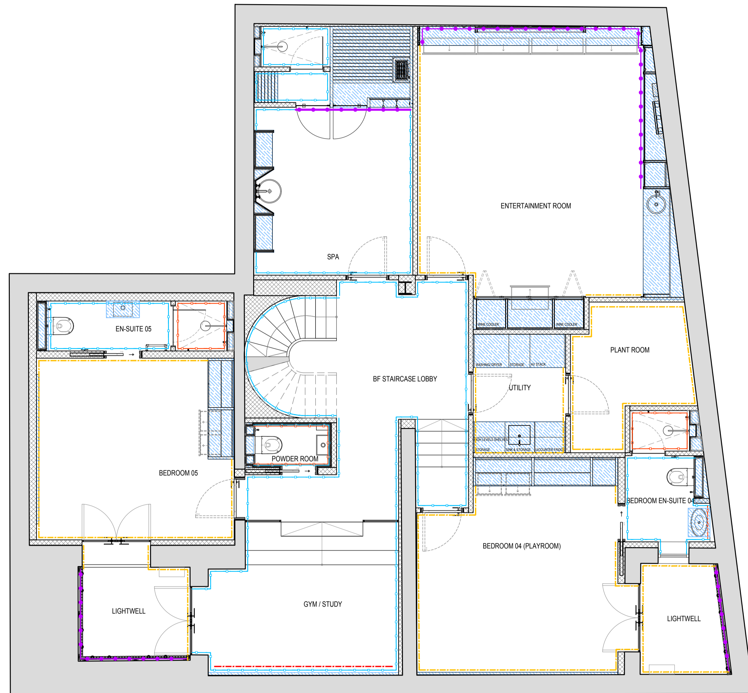
00 BF WALL FINISHES PLAN Scale 1:50
