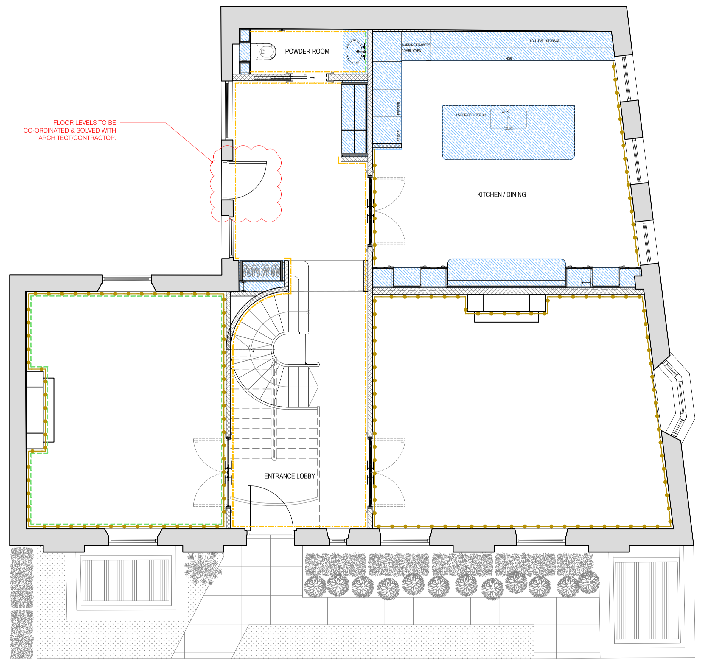
00 GF WALL FINISHES PLAN Scale 1:50
